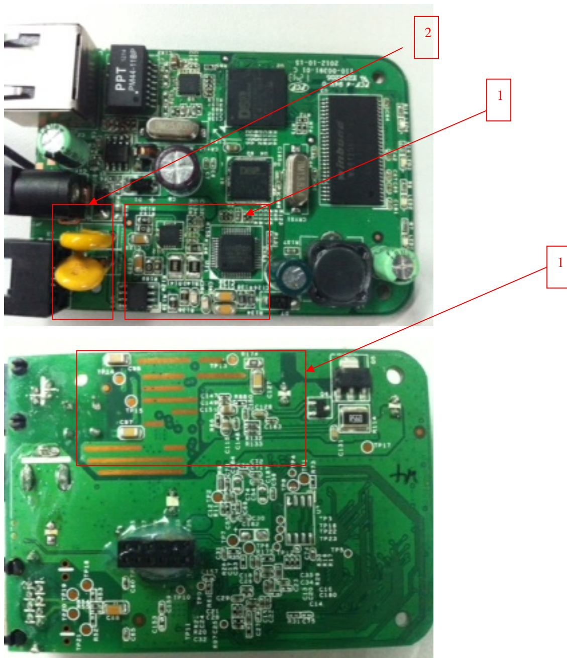
Original mainboard photo view
