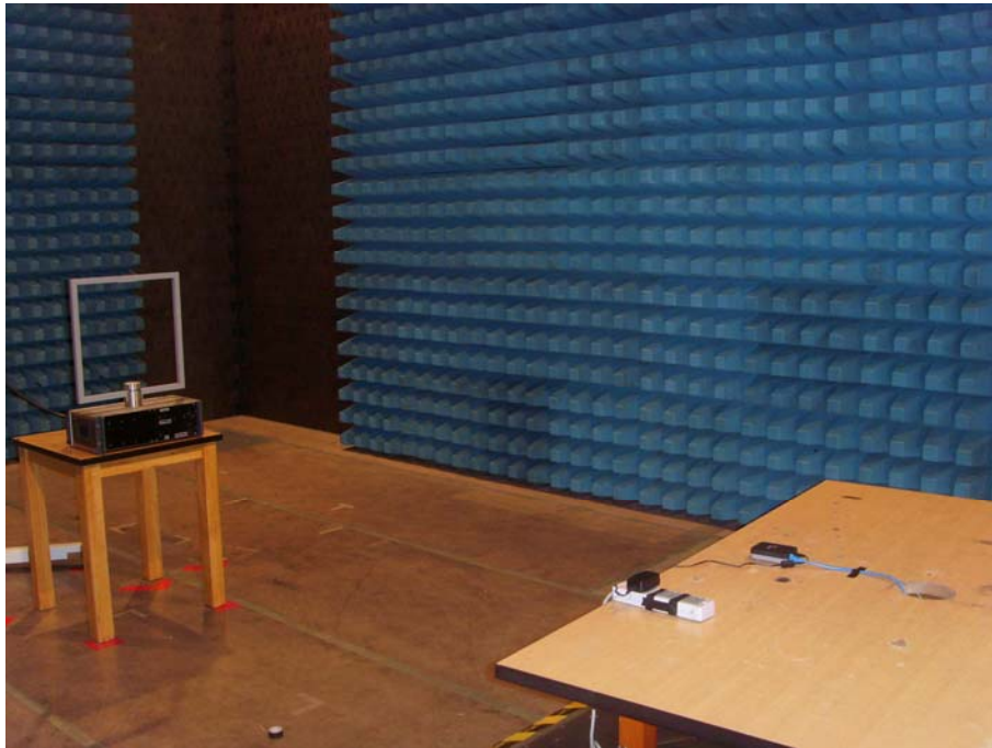
Radiated Emission Test Set-up(9kHz to 30MHz)
