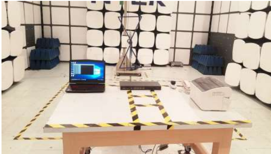
Radiated Emission Test Set-up(30-1000MHz)
