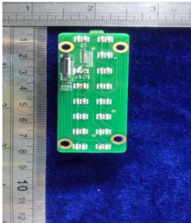
LED display board-Top view
