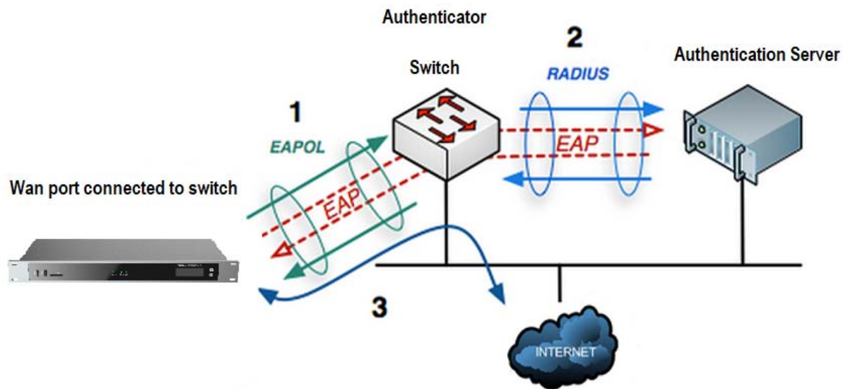
Figure 19: GXW450X Using 802.1X as Client
