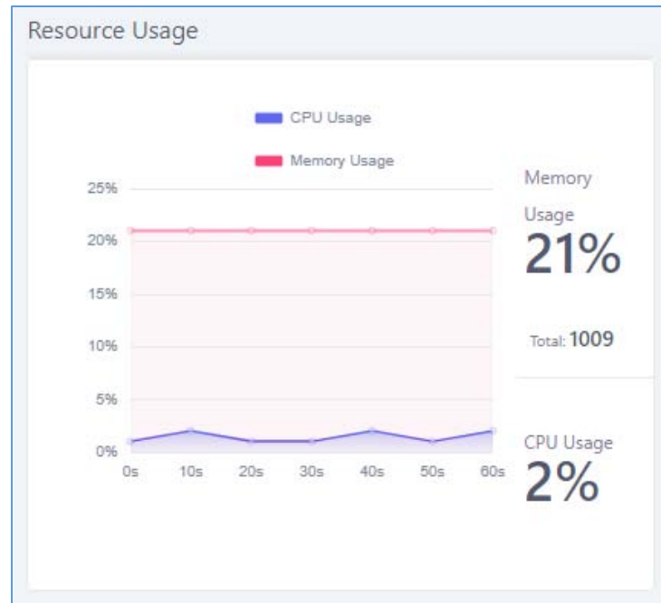
Figure 8: Resource Usage
