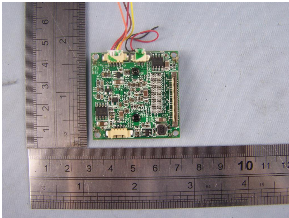
Sensor board - Top View
