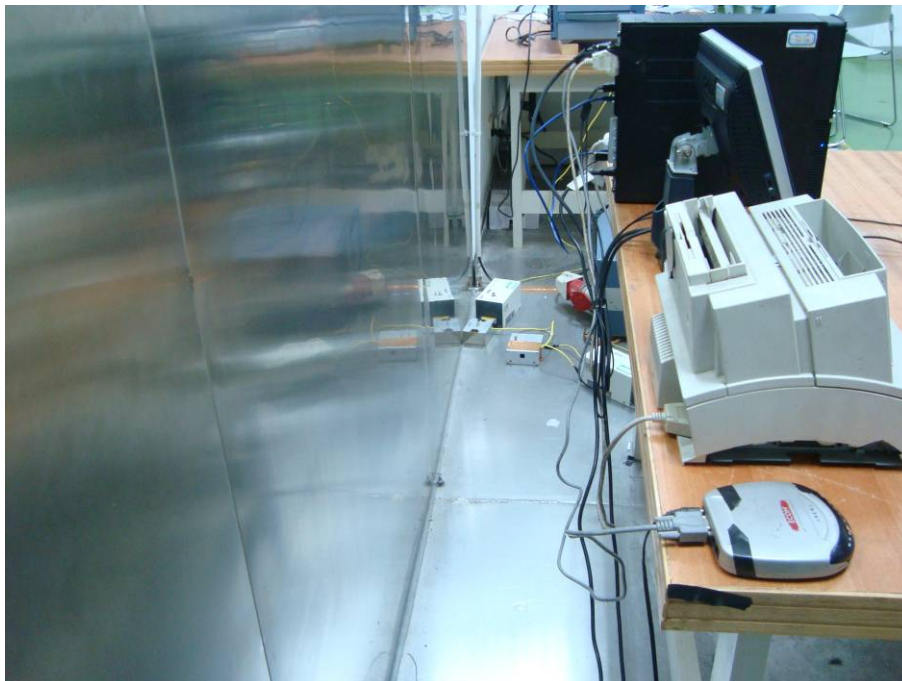
Conducted Disturbance at Mains Terminals - Side View
