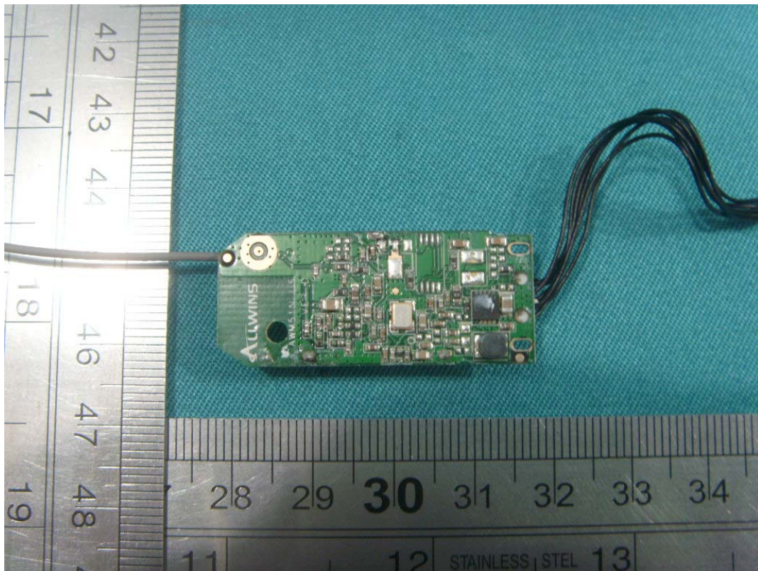
Wifi PCB Rear view
