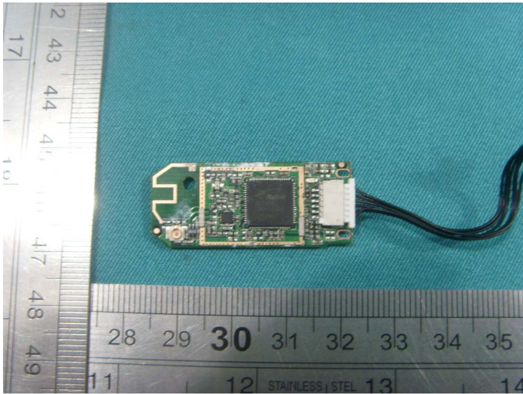
Wifi PCB front view(removed shield cover)
