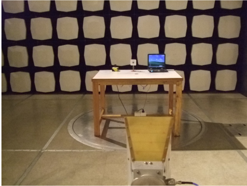
Radiated Emission Test Set-up - Above
