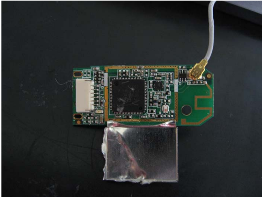
802.11b/g/n module -Unshield View
