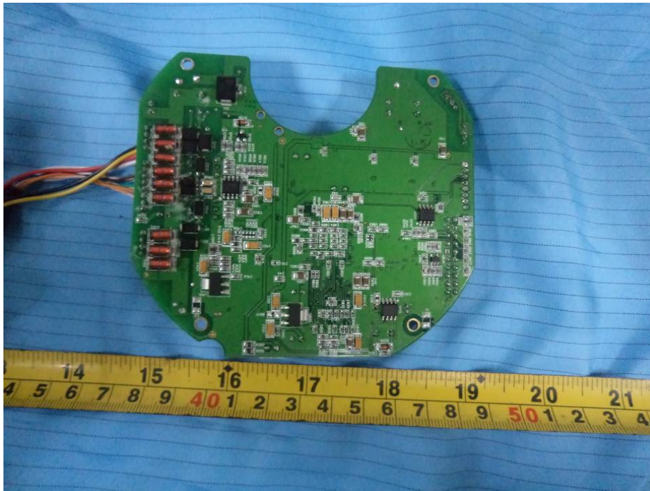
EUT – GXV3612-U02A Board Bottom View
