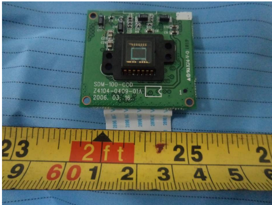
EUT – SDM-100-CCD Board Bottom View
