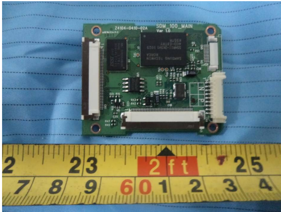
EUT – SDM-100-MAIN Board Bottom View
