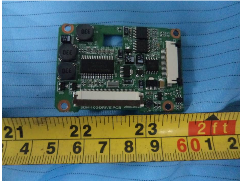
EUT – SDM-100-Drive Board Bottom View
