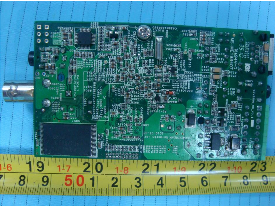
EUT –MS-ME198407 Board Top View
