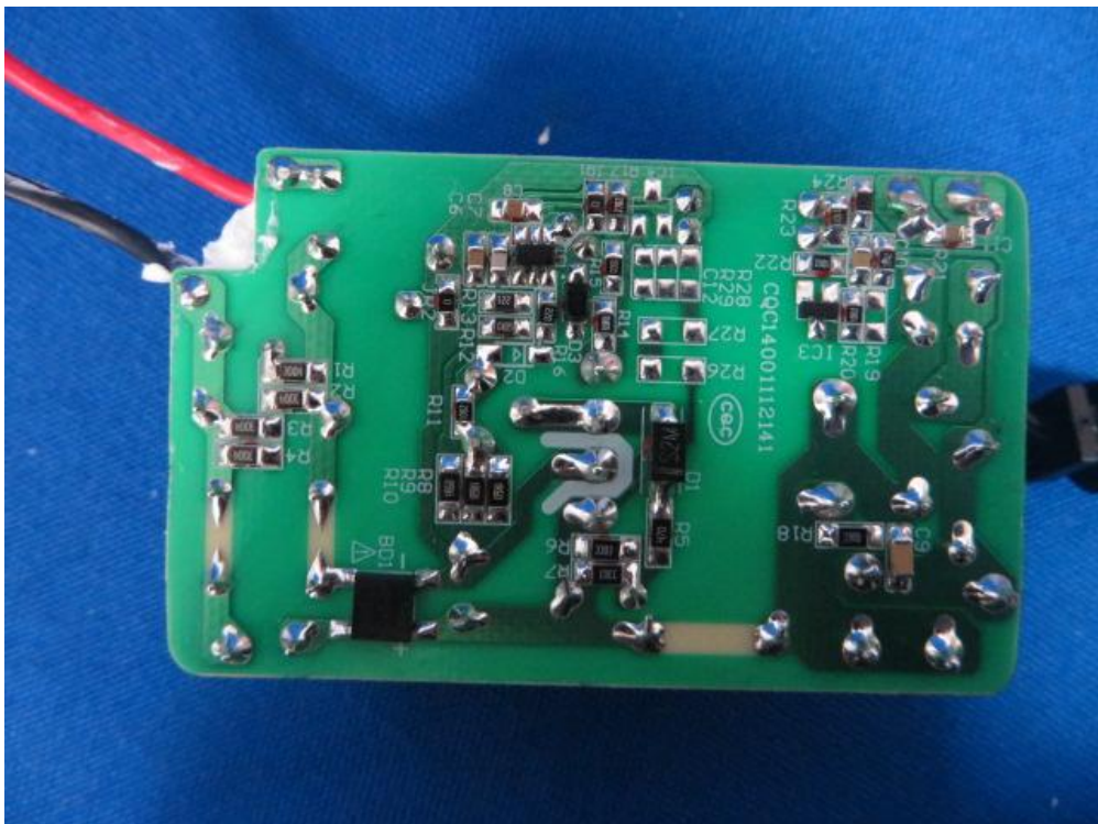
(8) EUT Photo (M/N: F18W8-120150SPAUY)
