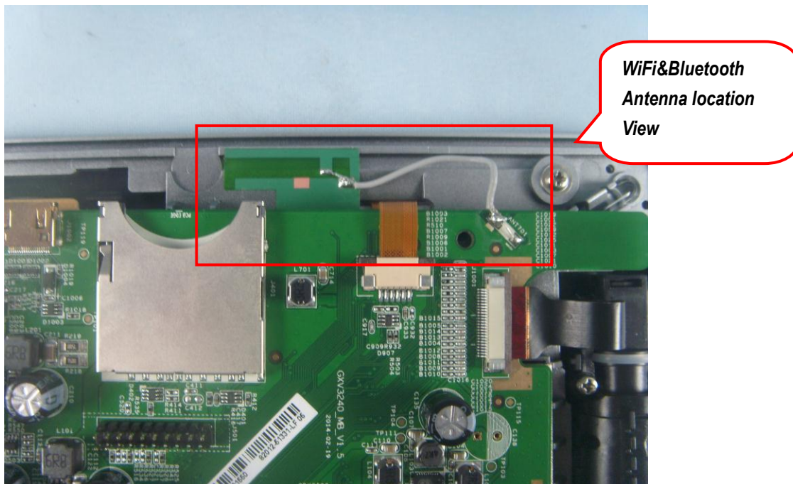
Main board View
