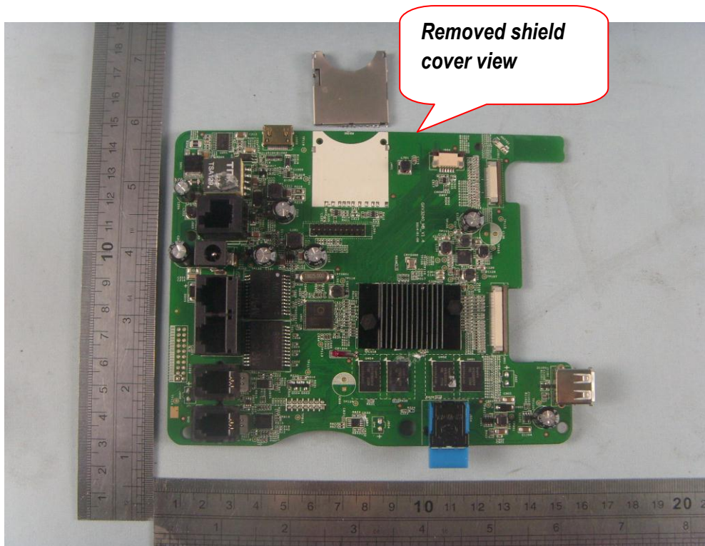
Main board- Top View #2
