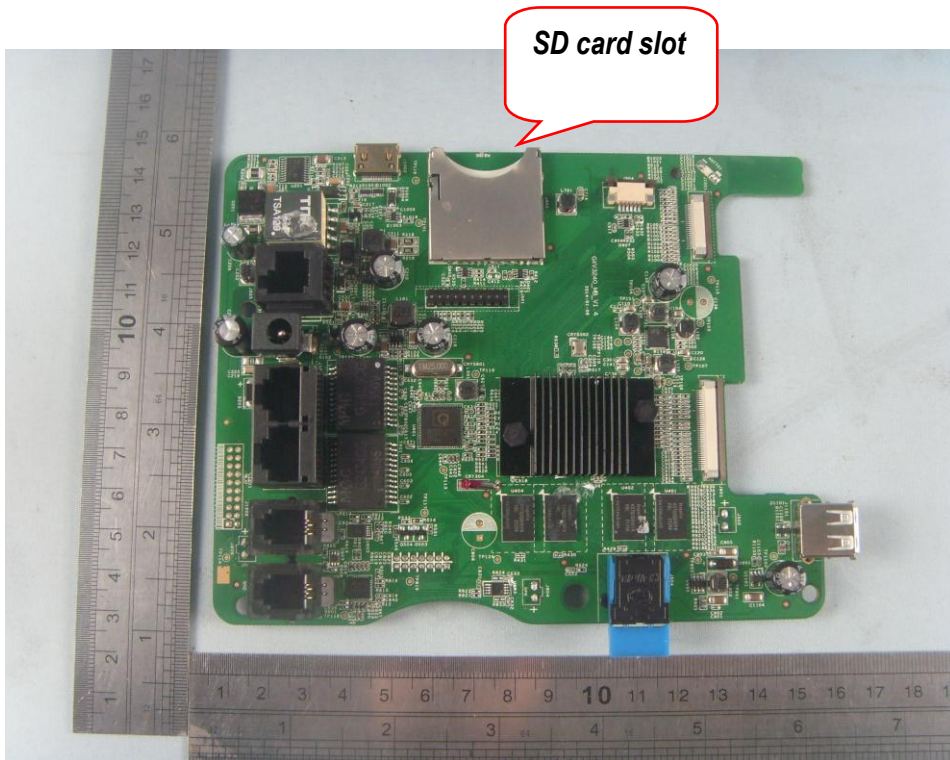
Main board- Top View #1
