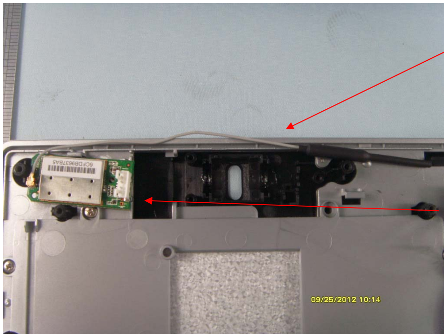
Wi-Fi module plus antenna view
