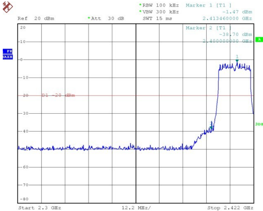
Conducted Band Edge Test Plot: 2412MHz
