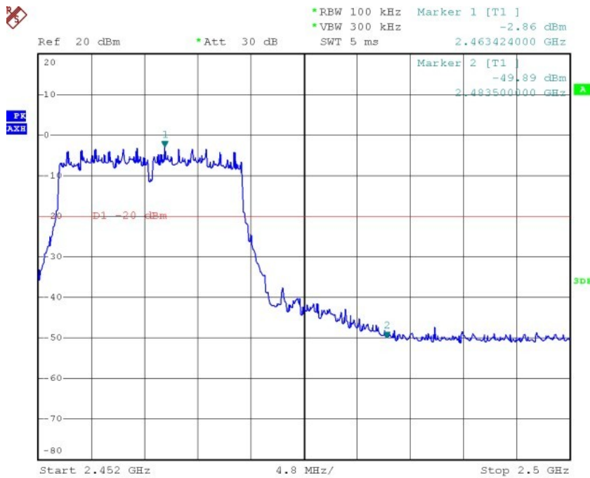
Conducted Band Edge Test Plot: 2462MHz
