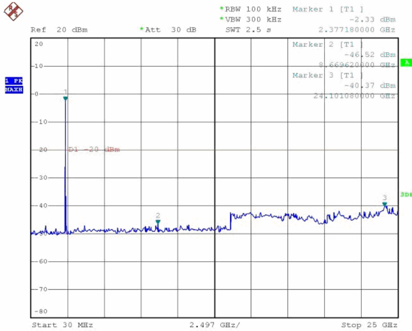
Low Channel: 2412MHz
