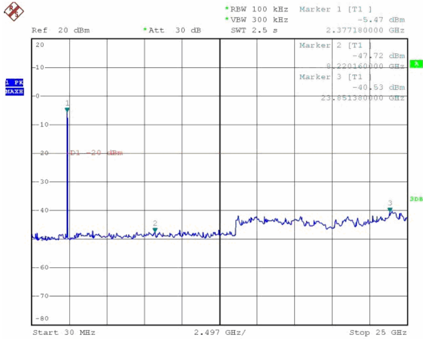
Low Channel: 2422MHz
