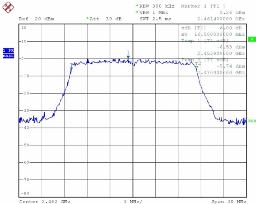
High Channel: 2462MHz
