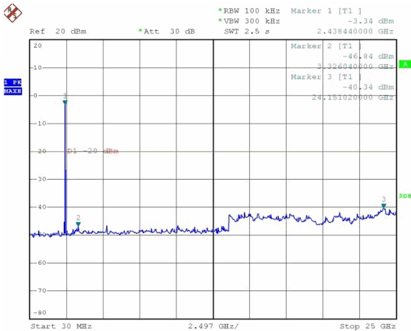
Mid Channel: 2437MHz
