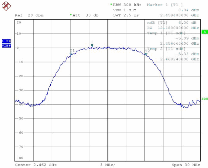
High Channel: 2462MHz
