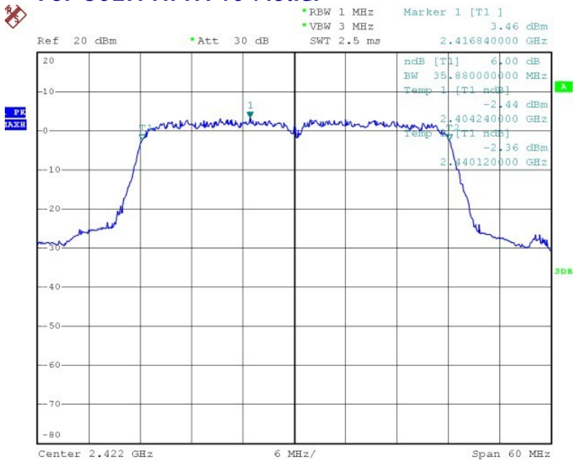
Low Channel: 2422MHz
