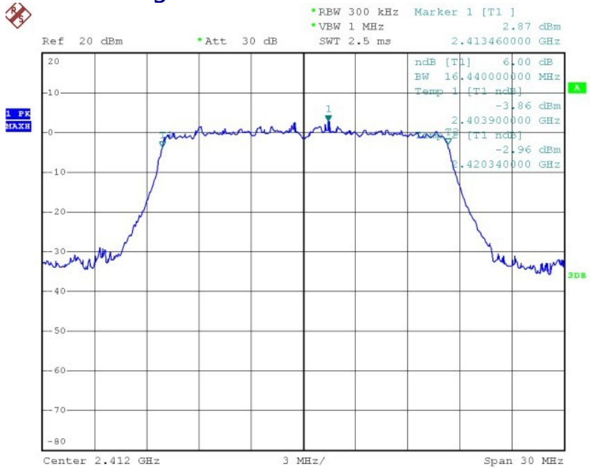
Low Channel: 2412MHz
