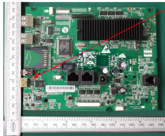
GXV3174 front view for Version 2.6
