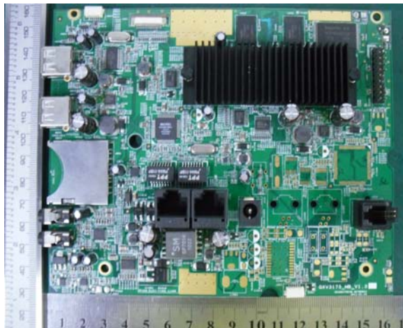
GXV3174 front view for Version 1.3
