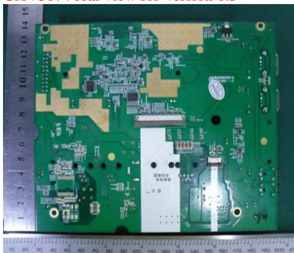
GXV3174 rear view for Version 1.3
