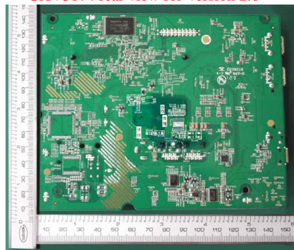
GXV3174 rear view for Version 2.6
