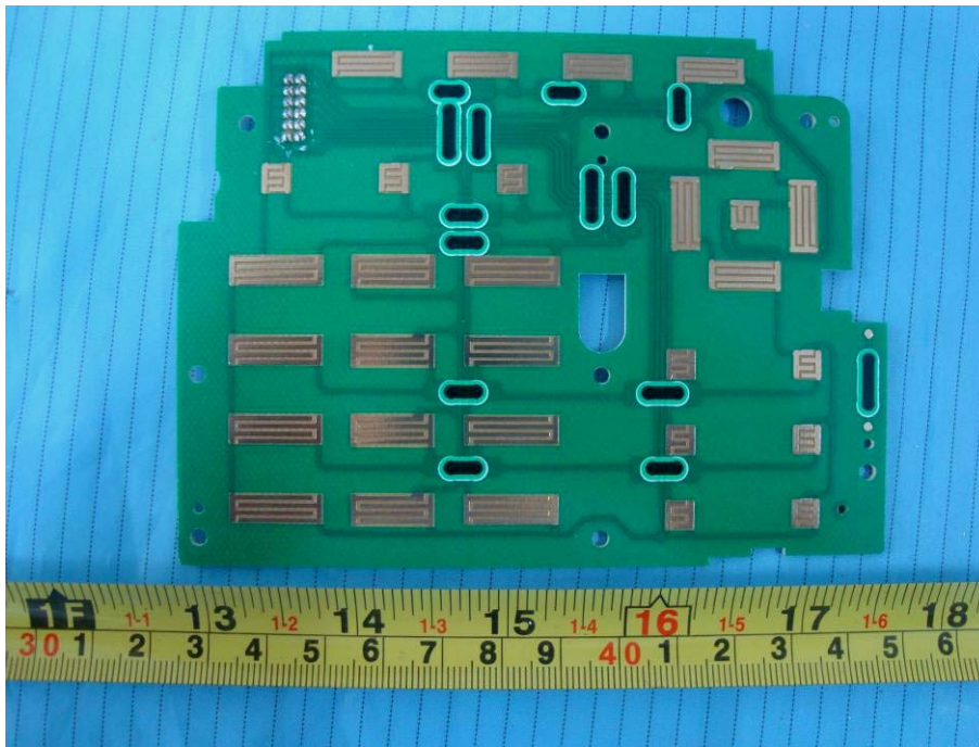
EUT – Handset Top View
