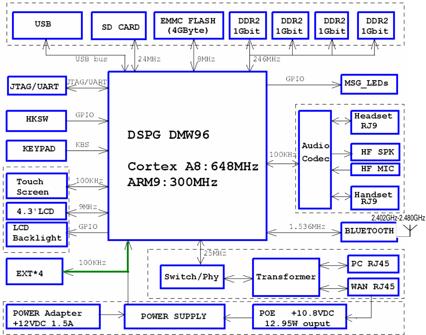
GXP2200 System Block Diagram
