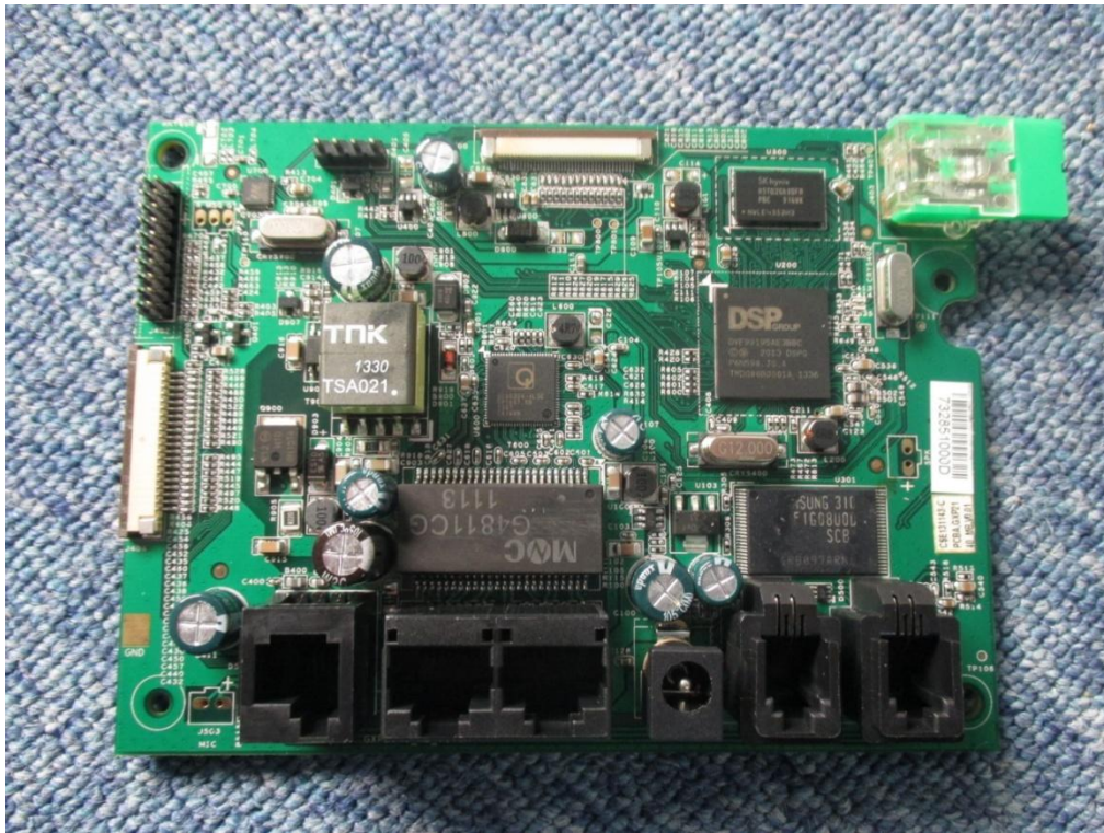
Main board GXP2140_MB_V1.5A
