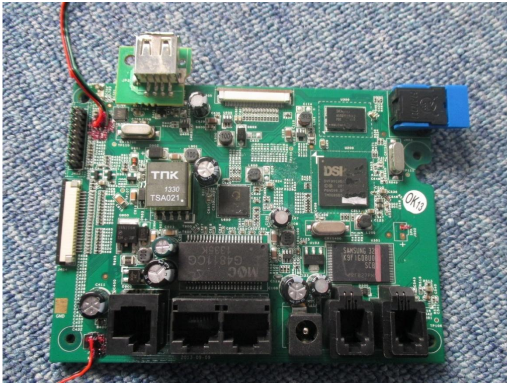
Main board GXP2140_MB_V1.4A
