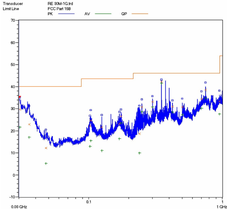
Horizontal: Radiated Emission Test Plot (Peak,maxhold)- Power Adaptor #1(Mass power)
