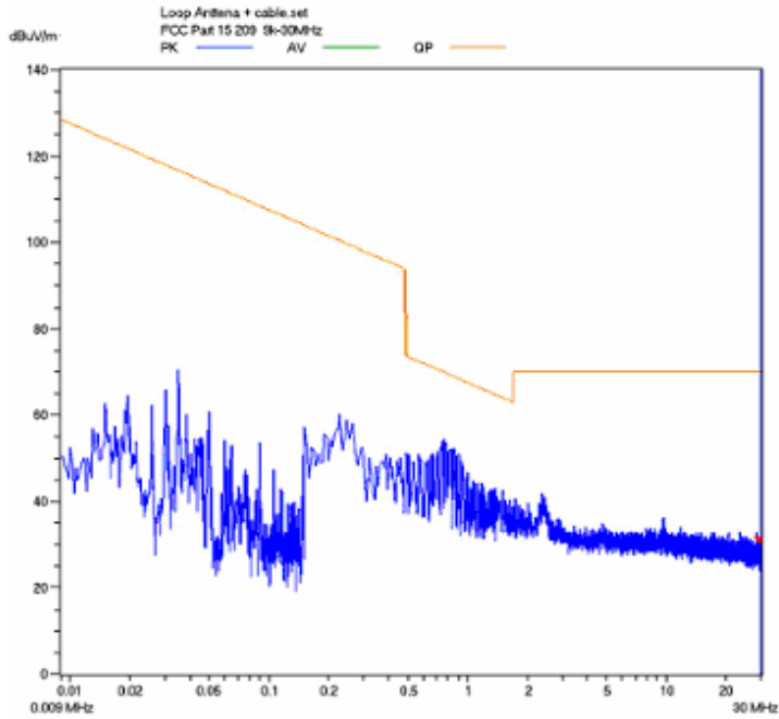
Radiated Filed Strength Emission Test Plot (Peak,maxhold)-Power Adapter #1
