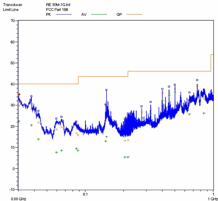
Vertical: Radiated Emission Test Plot (Peak,maxhold) Power Adaptor #2(UE Power)
