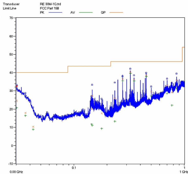
Horizontal: Radiated Emission Test Plot (Peak,maxhold) Power Adaptor #2(UE Power)
