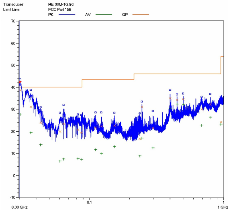
Vertical: Radiated Emission Test Plot (Peak,maxhold) Power Adaptor #1(Mass power)
