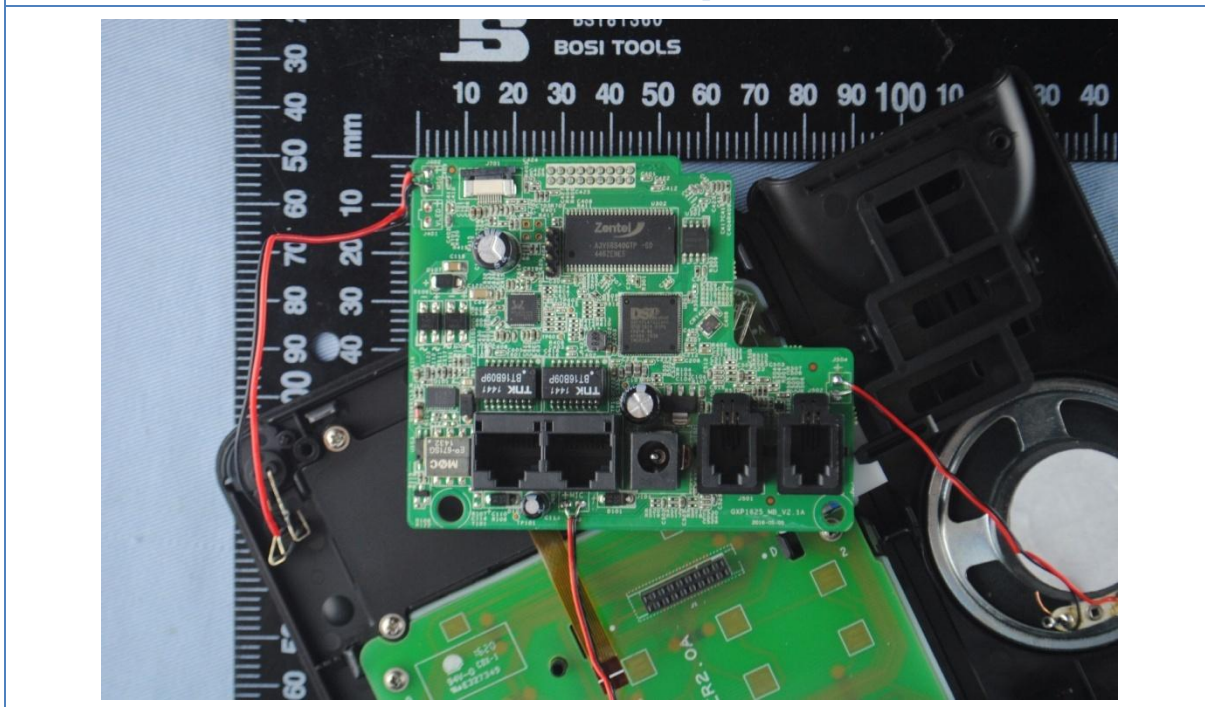
GXP165 Main board component side
