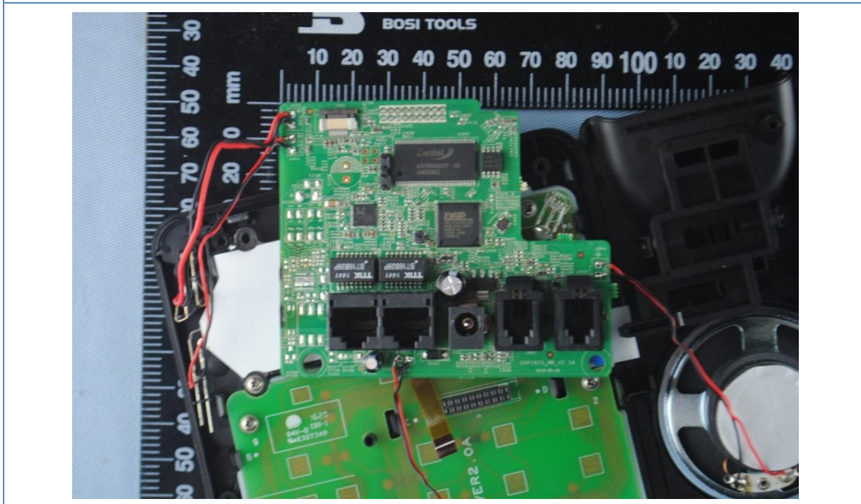
GXP1620 Main board component side
