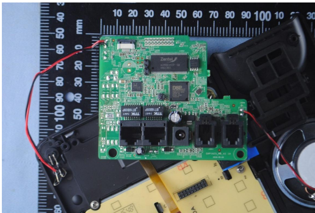
GXP1610 Main board component side
