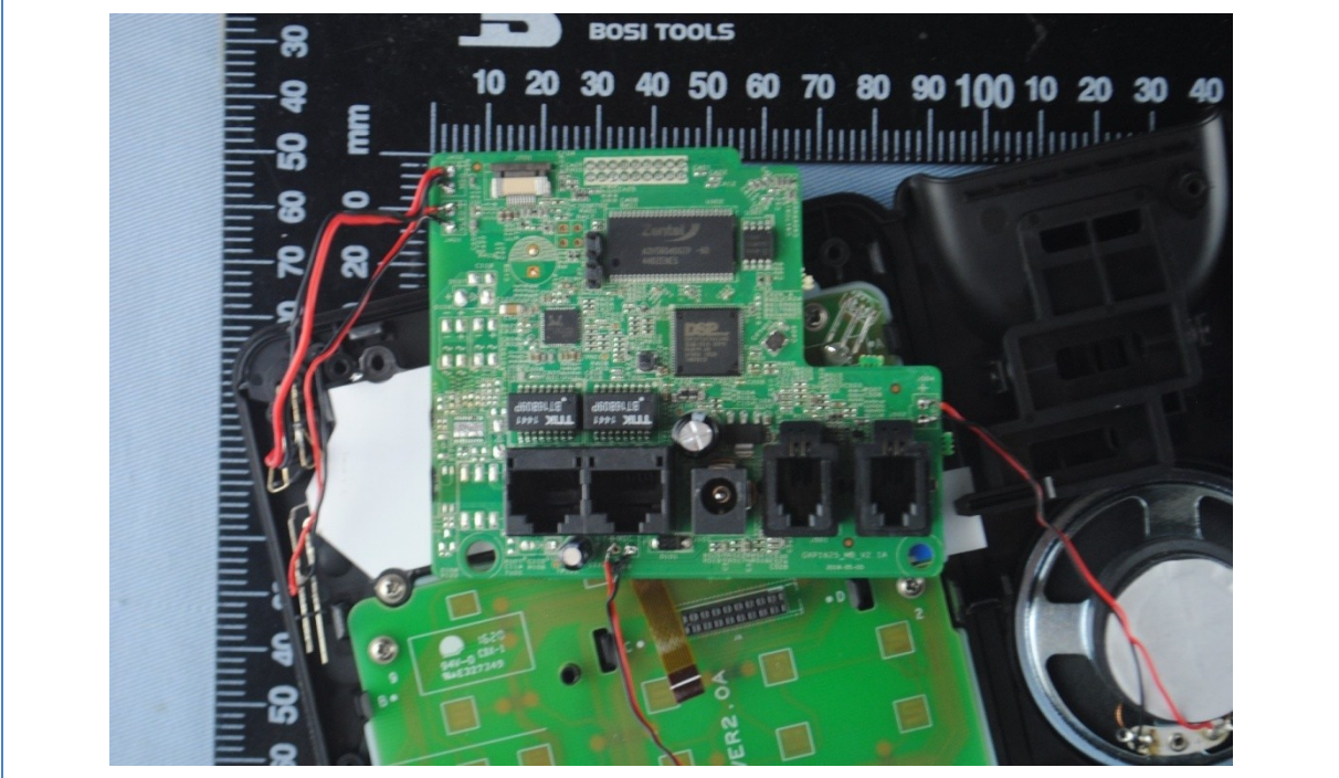
GXP1620 Main board component side
