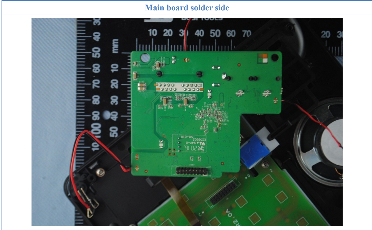
GXP1610 Main board component side
