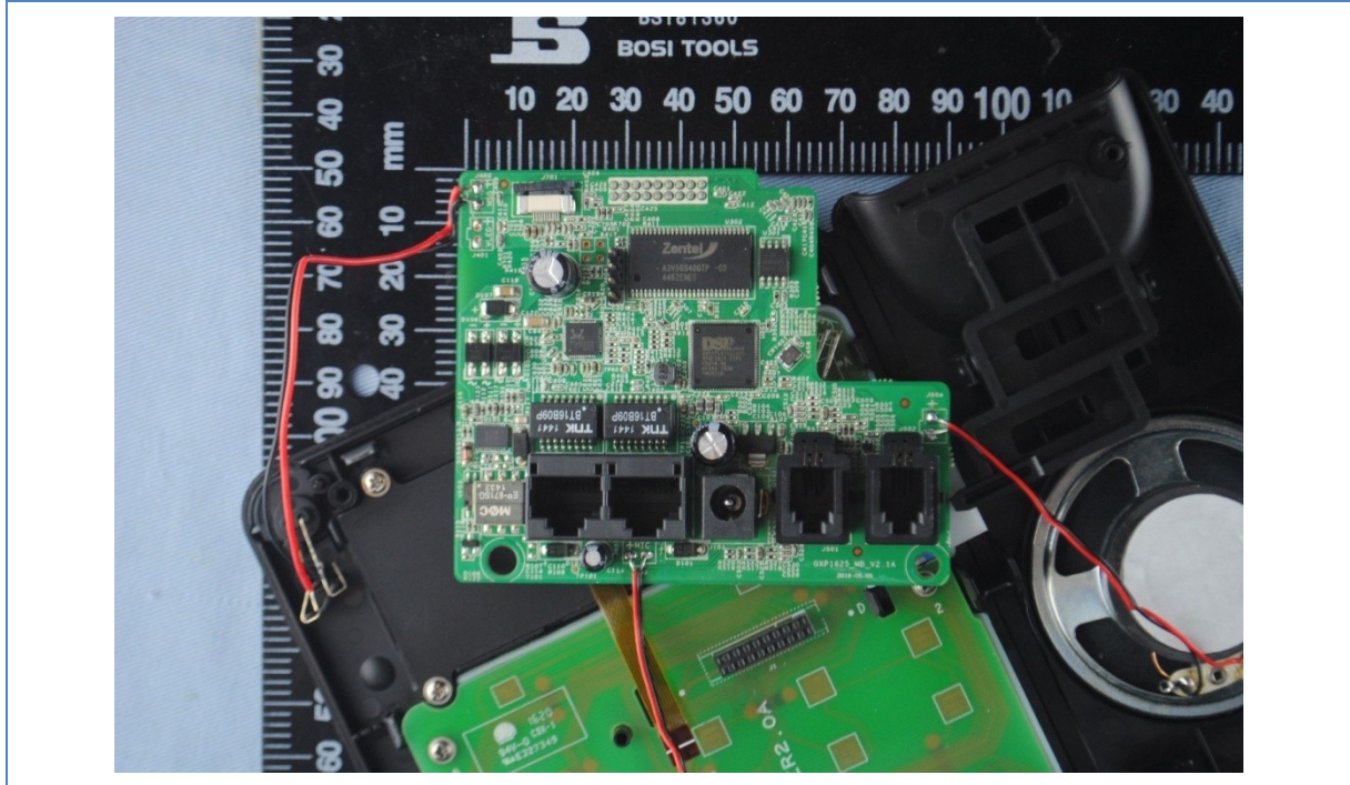
GXP1615 Main board component side
