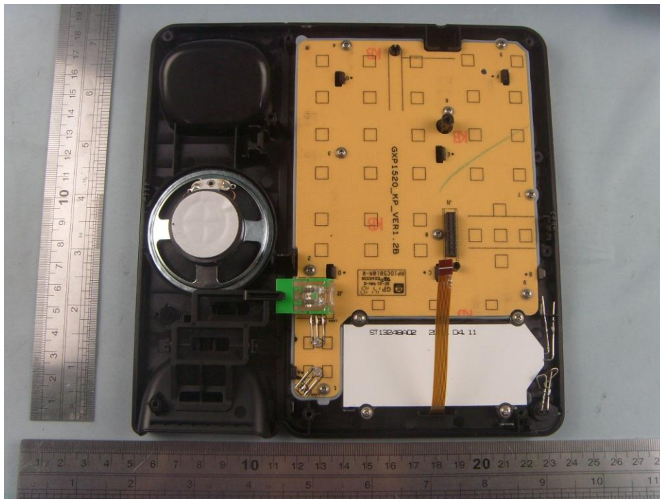
EUT-Uncovered View #2
