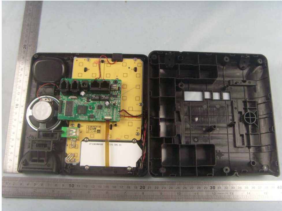
EUT-Uncovered View #1
