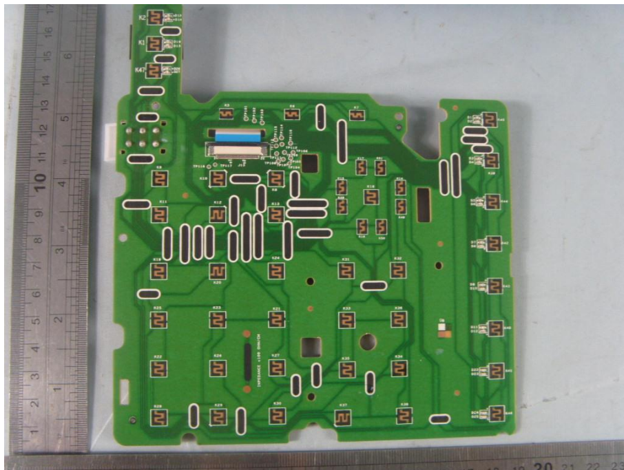
Key-board-Top view
