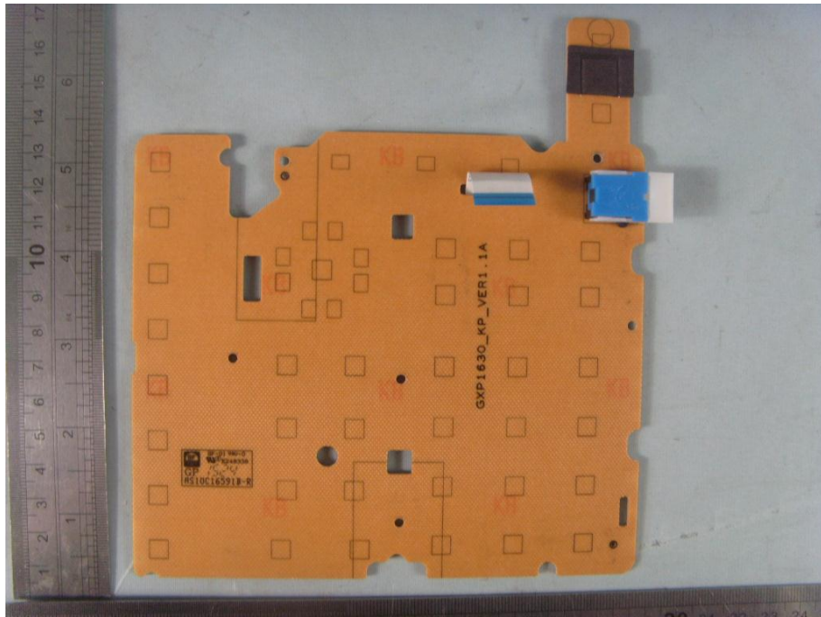
Key-board-Bottom view
