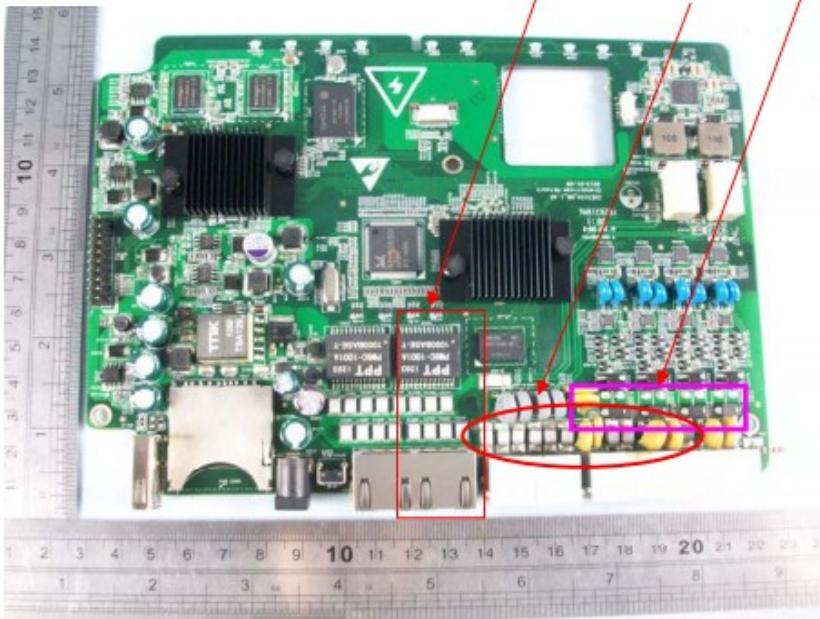
New mainboard photo view
