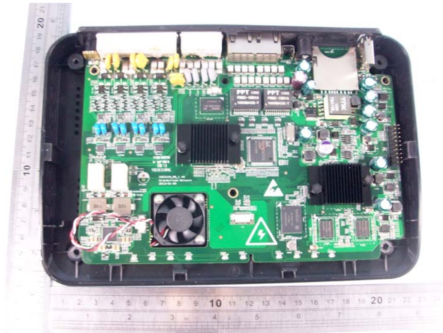
EUT-Uncovered View
