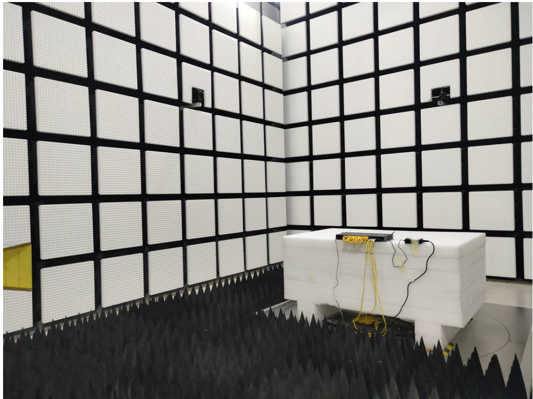
Radiated Emissions Above 1G Rear View-M3
