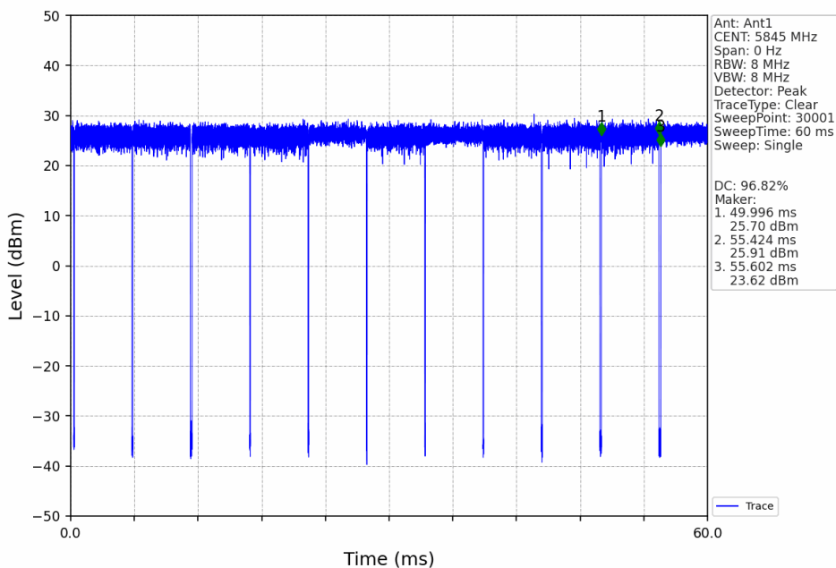
802.11n(HT20)_HCH_5845MHz_Ant1_NTNV
