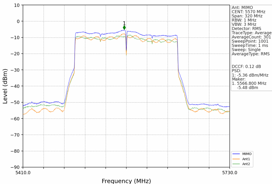
802.11ax(HEW160)_MCH_5570MHz_SU_MIMO_NTNV
