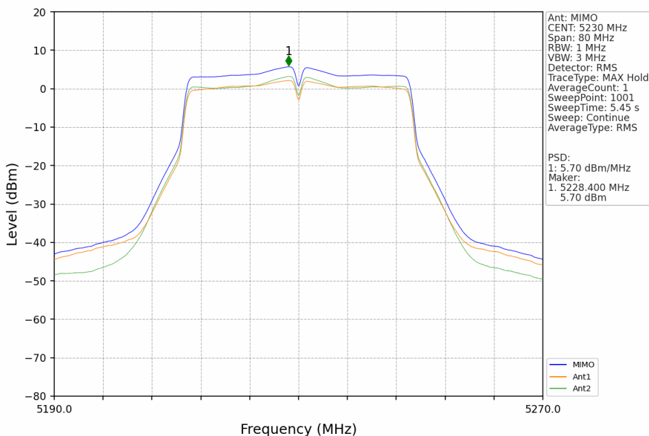
802.11ac(VHT40)_HCH_5230MHz_MIMO_NTNV
