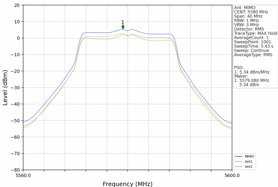
802.11ac(VHT20)_MCH_5580MHz_MIMO_NTNV
