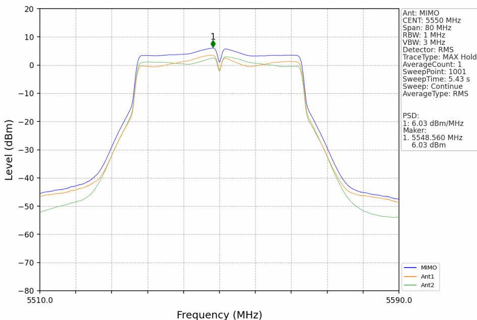
802.11ac(VHT40)_MCH_5550MHz_MIMO_NTNV
