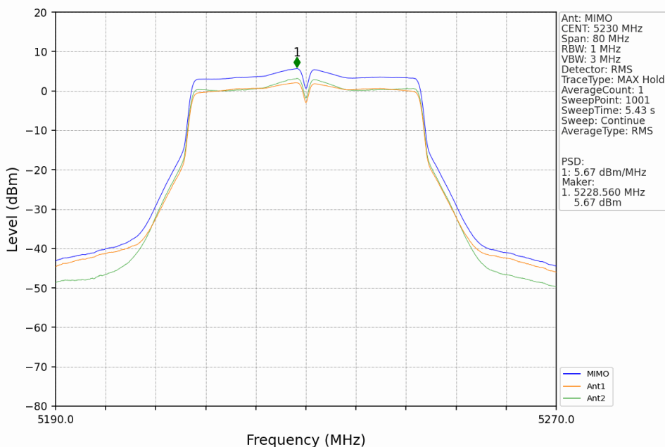
802.11n(HT40)_HCH_5230MHz_MIMO_NTNV
