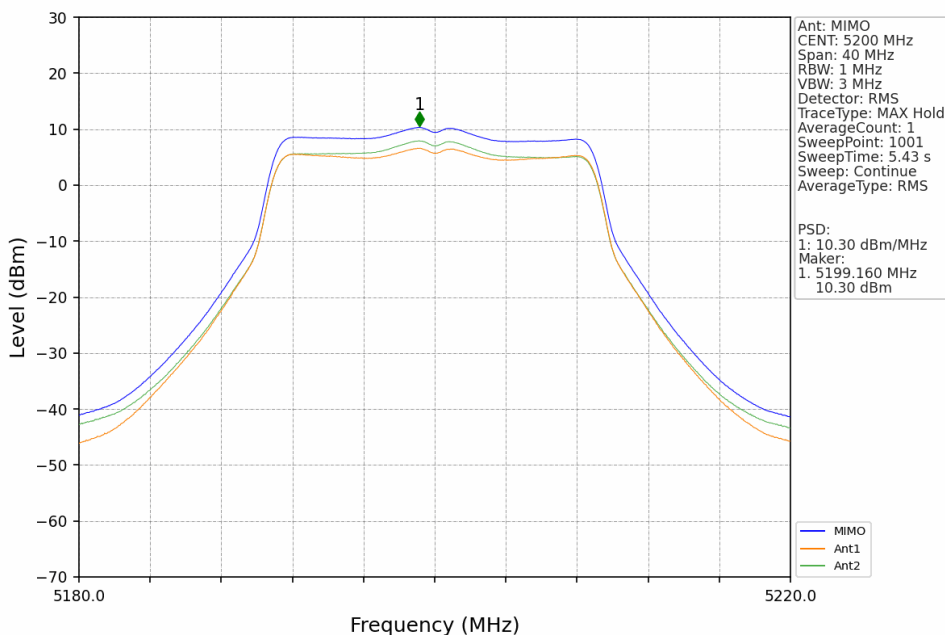
802.11ac(VHT20)_MCH_5200MHz_MIMO_NTNV
