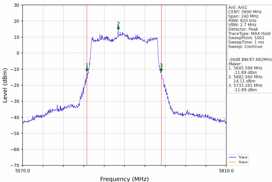
802.11ax(HEW80)_HCH_5690MHz_SU_Ant1_NTNV
