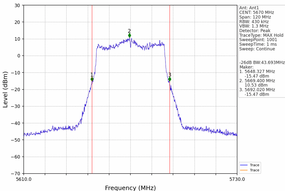
802.11ax(HEW40)_HCH_5670MHz_SU_Ant1_NTNV
