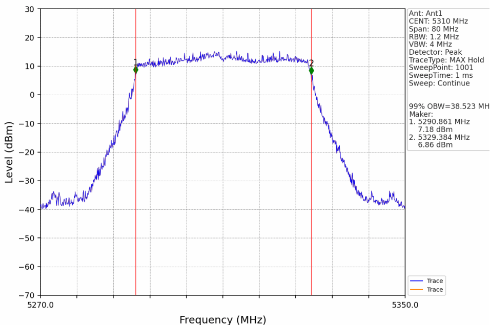
802.11ax(HEW40)_HCH_5310MHz_SU_Ant1_NTNV
