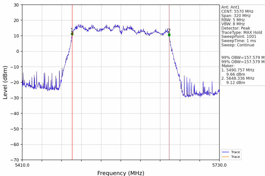
802.11ac(VHT160)_MCH_5570MHz_Ant1_NTNV
