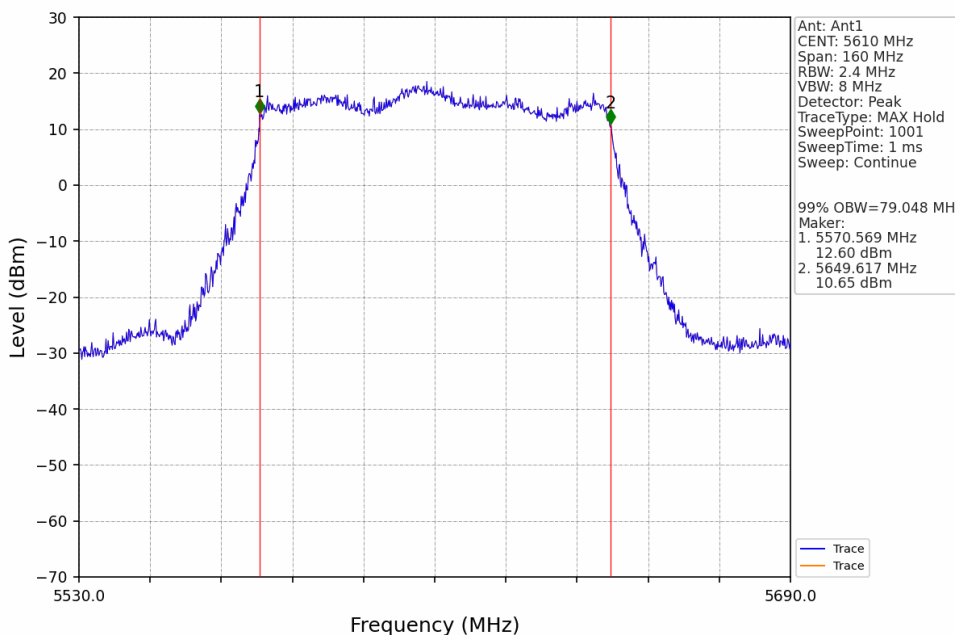
802.11ax(HEW80)_HCH_5610MHz_SU_Ant1_NTNV
