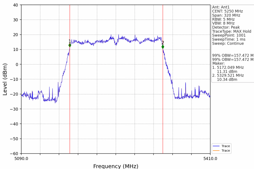
802.11ac(VHT160)_MCH_5250MHz_Ant1_NTNV
