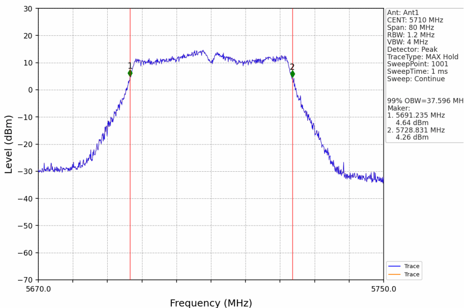
802.11ac(VHT40)_HCH_5710MHz_Ant1_NTNV
