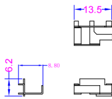
5G Antenna
