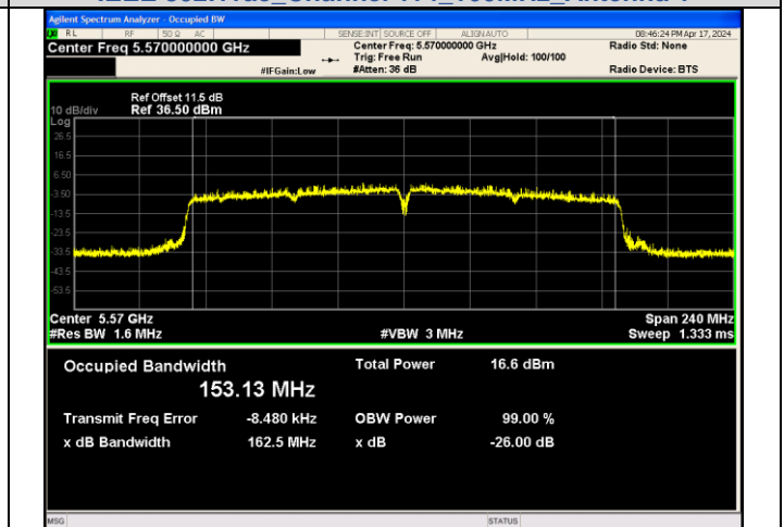
IEEE 802.11ac_Channel 114_160MHz_Antenna 3
