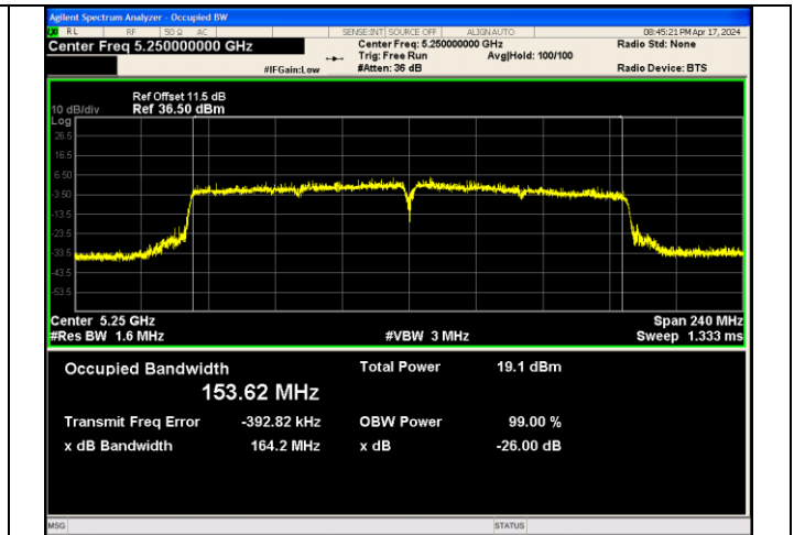
IEEE 802.11ac_Channel 50_160MHz_Antenna 3
