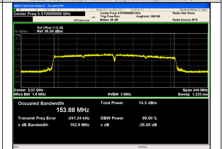
IEEE 802.11ac_Channel 114_160MHz_Antenna 1
