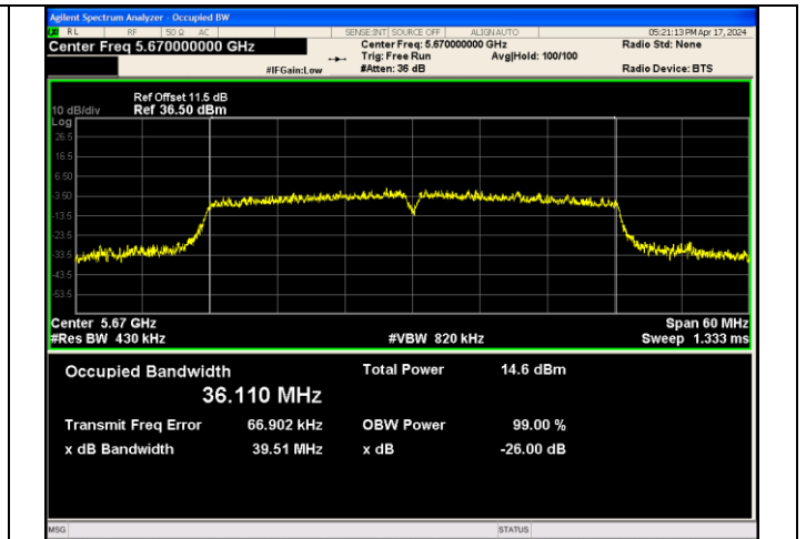
IEEE 802.11ac_Channel 134_40MHz_Antenna 1
