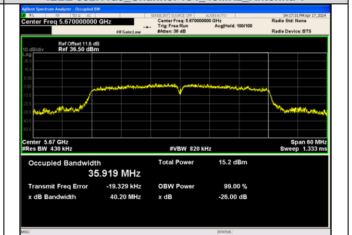
IEEE 802.11ac_Channel 134_40MHz_Antenna 3
