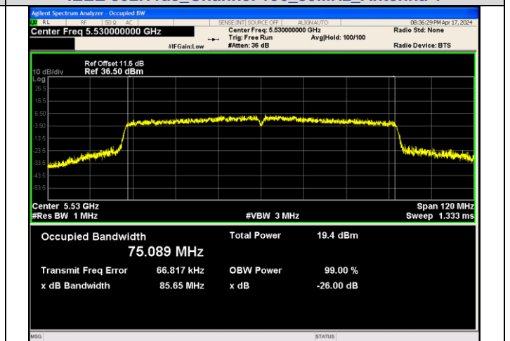
IEEE 802.11ac_Channel 106_80MHz_Antenna 3
