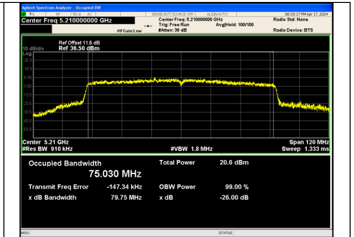
IEEE 802.11ac_Channel 42_80MHz_Antenna 3
