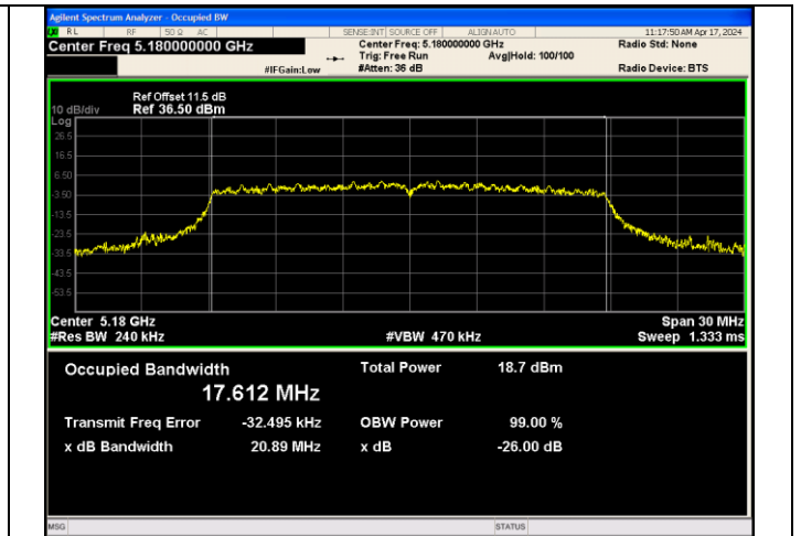
IEEE 802.11ac_Channel 36_20MHz_Antenna 1
