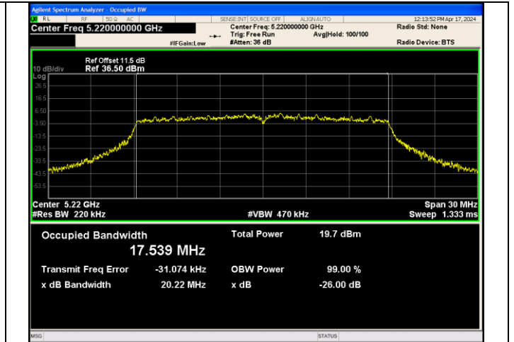
IEEE 802.11ac_Channel 44_20MHz_Antenna 3
