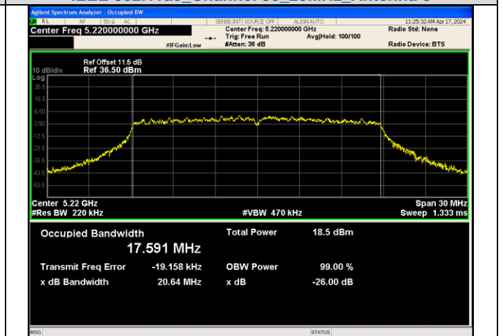
IEEE 802.11ac_Channel 44_20MHz_Antenna 1
