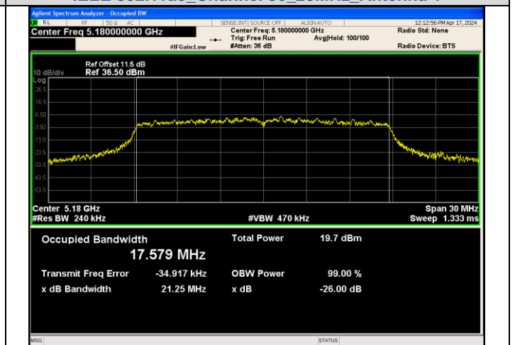
IEEE 802.11ac_Channel 36_20MHz_Antenna 3
