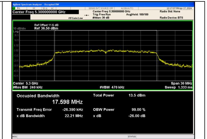
IEEE 802.11ac_Channel 60_20MHz_Antenna 3
