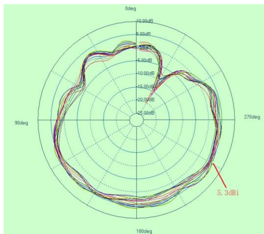
Elevation angle above 30 degrees
