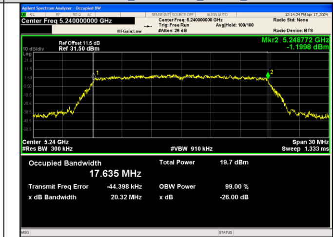
IEEE 802.11ac_Channel 48_20MHz_Antenna 3
