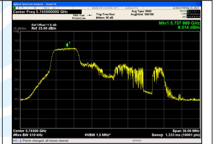
IEEE 802.11ax_Channel 149_20MHz_Antenna 1_RU&Index 26RU
