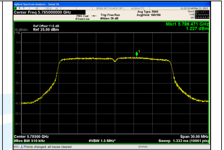
IEEE 802.11ac_Channel 157_20MHz_Antenna 3
