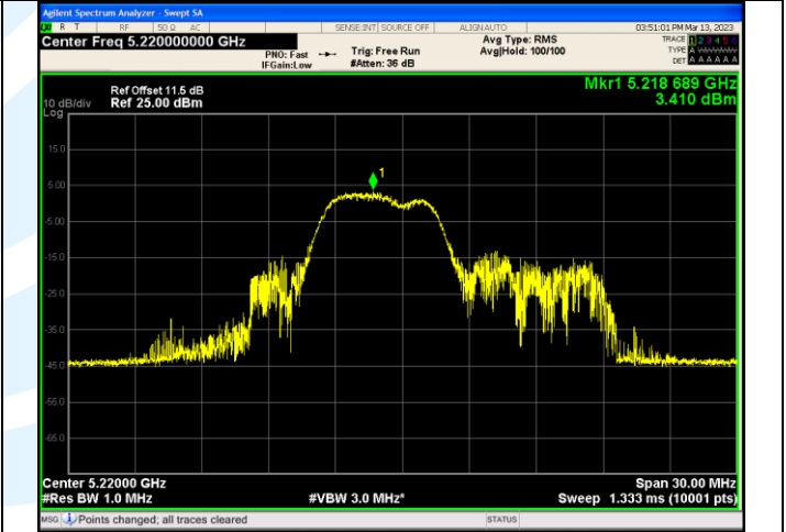
IEEE 802.11ax_Channel 44_20MHz_Antenna 1_RU&Index 26RU4
