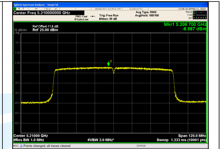
IEEE 802.11ac_Channel 42_80MHz_Antenna 1
