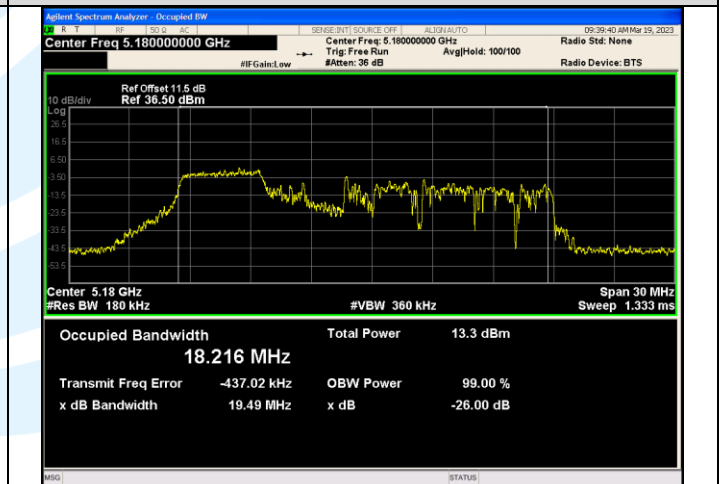
IEEE 802.11ax_Channel 36_20MHz_Antenna 3_RU&Index 26RU0
