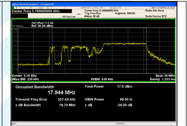
IEEE 802.11ax_Channel 36_20MHz_Antenna 1_RU&Index 26RU0
