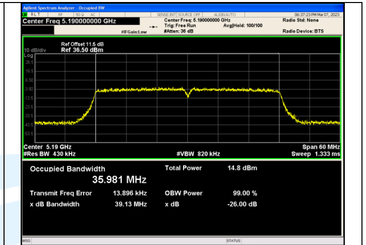
IEEE 802.11n_Channel 38_40MHz_Antenna 1
