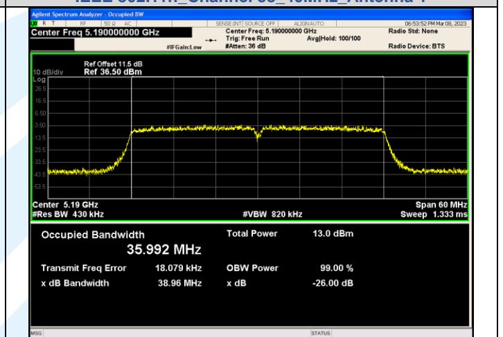
IEEE 802.11n_Channel 38_40MHz_Antenna 3
