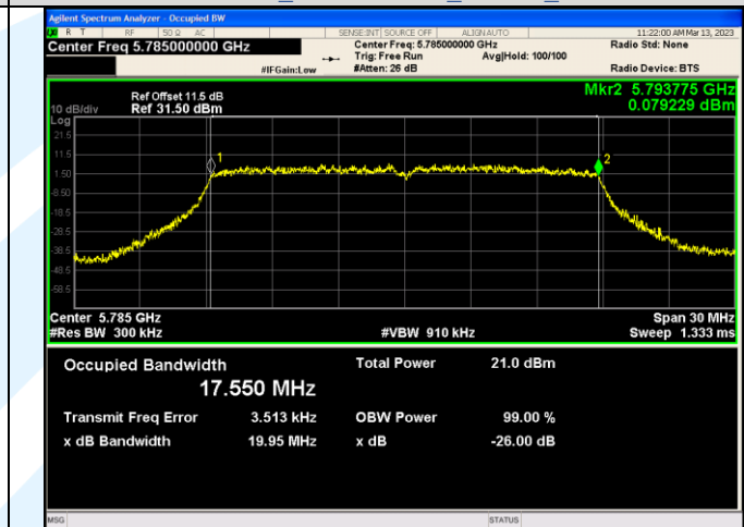
IEEE 802.11ac_Channel 157_20MHz_Antenna 3
