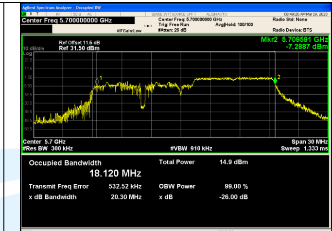
IEEE 802.11ax_Channel 140_20MHz_Antenna 1_RU&Index 52RU40
