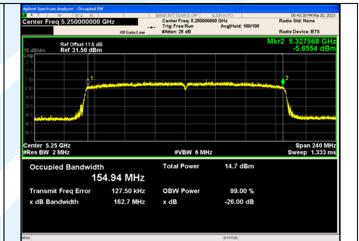
IEEE 802.11ac_Channel 50_80+80MHz_Antenna 1
