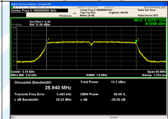
IEEE 802.11n_Channel 38_40MHz_Antenna 3
