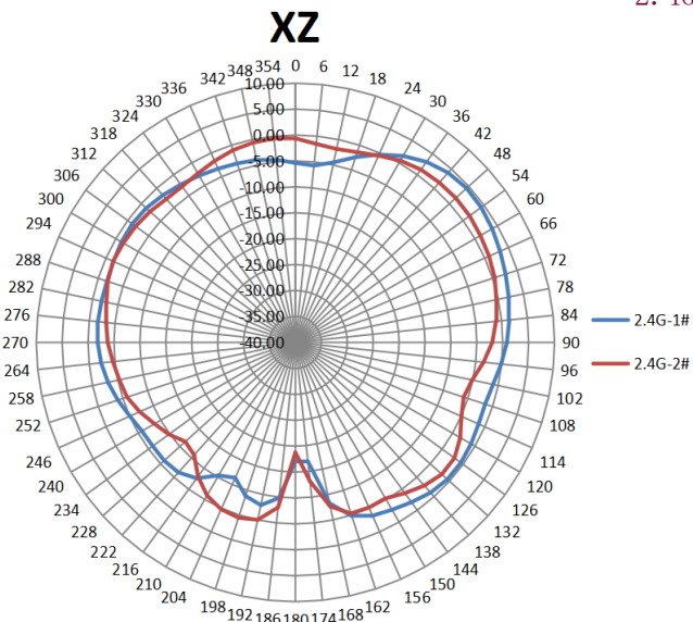
2.4G 辐射方向图 Radiation Patterns (unit: dB) 2.4G-1# 2480MHz 2.4G-2# 2450MHz
