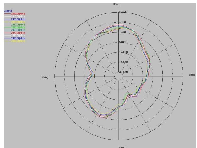
2.4G phi=90deg
