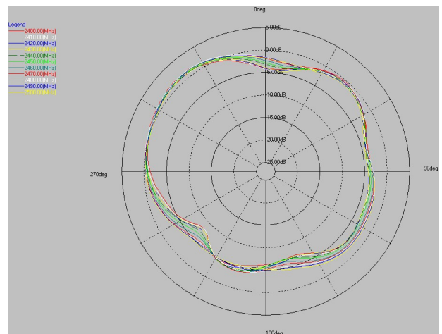
2.4G phi=90deg
