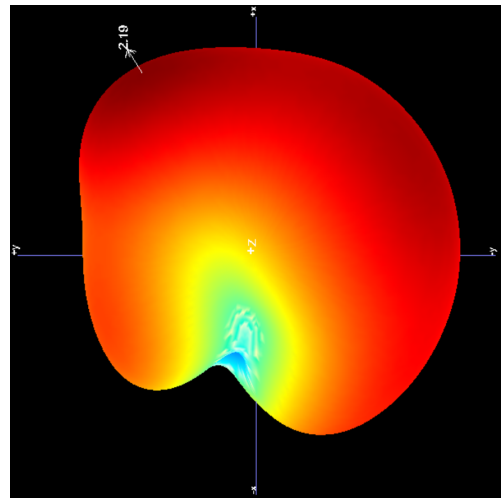
2.4G 3D
