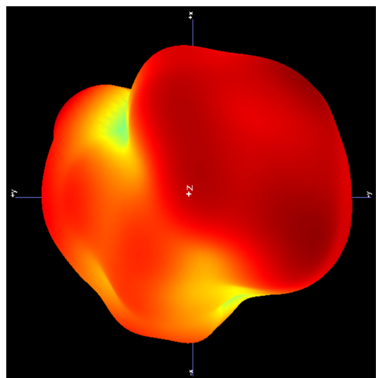
5G 3D
