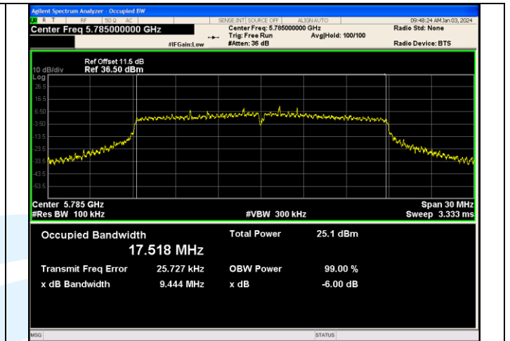
IEEE 802.11ac_Channel 157_20MHz_Antenna 1
