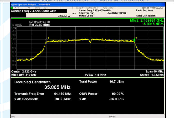
IEEE 802.11n_Channel 3_40MHz_Antenna 1
