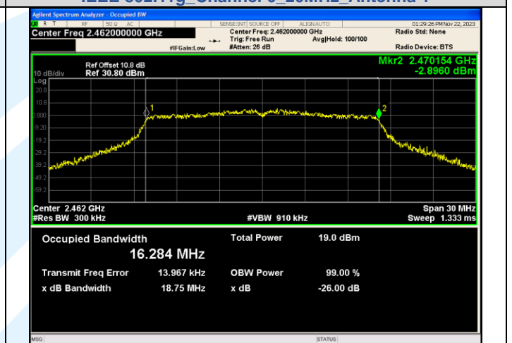
IEEE 802.11g_Channel 11_20MHz_Antenna 1
