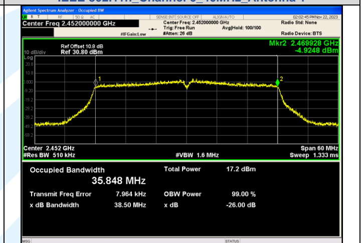
IEEE 802.11n_Channel 9_40MHz_Antenna 1
