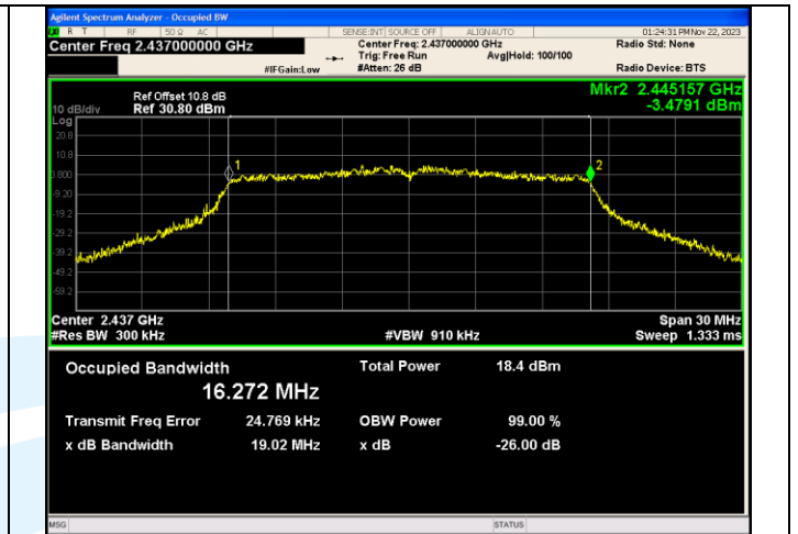
IEEE 802.11g_Channel 6_20MHz_Antenna 1
